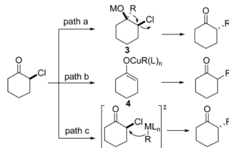
Scheme 2. Potential Reaction Mechanisms
